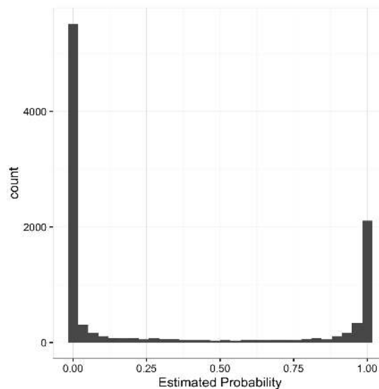
Figure 3: A histogram of probability estimates produced by AdaBoost on the two-dimensional circle example . The probability estimates are pushed to the extremes of 0 and 1.
