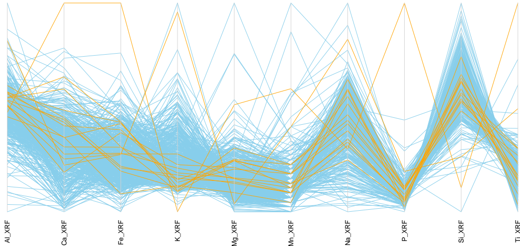
Figure 23: Parallel coordinate plot of the variables AL_{XRF} , Ca_{XRF} , Fe_{XRF} , K_{XRF} , Mg_{XRF} , Mn_{XRF} , Na_{XRF} , P_{XRF} , Si_{XRF} and Ti_{XRF} of the chorizon data set, imputed values in Bi are highlighted
