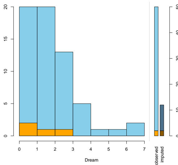
Figure 10: Customized histogram graphics of variable Dream of the data set sleep , imputed values in NonD and/or Sleep are highlighted
