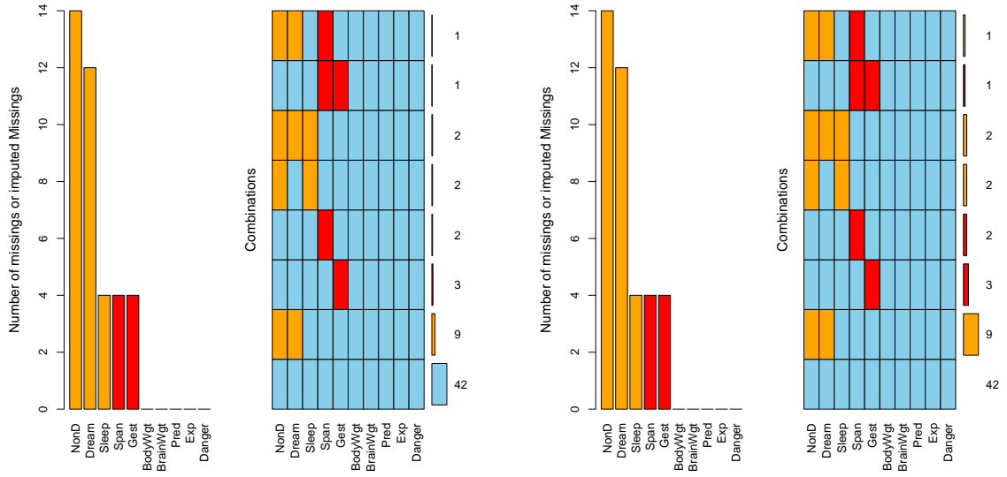
(a) Aggregation graphic with sorted variables and (b) Aggregation graphic showing only combinations with missing or imputed values in the right barplot
