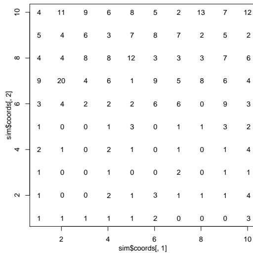
Figure 1: Simulated data
