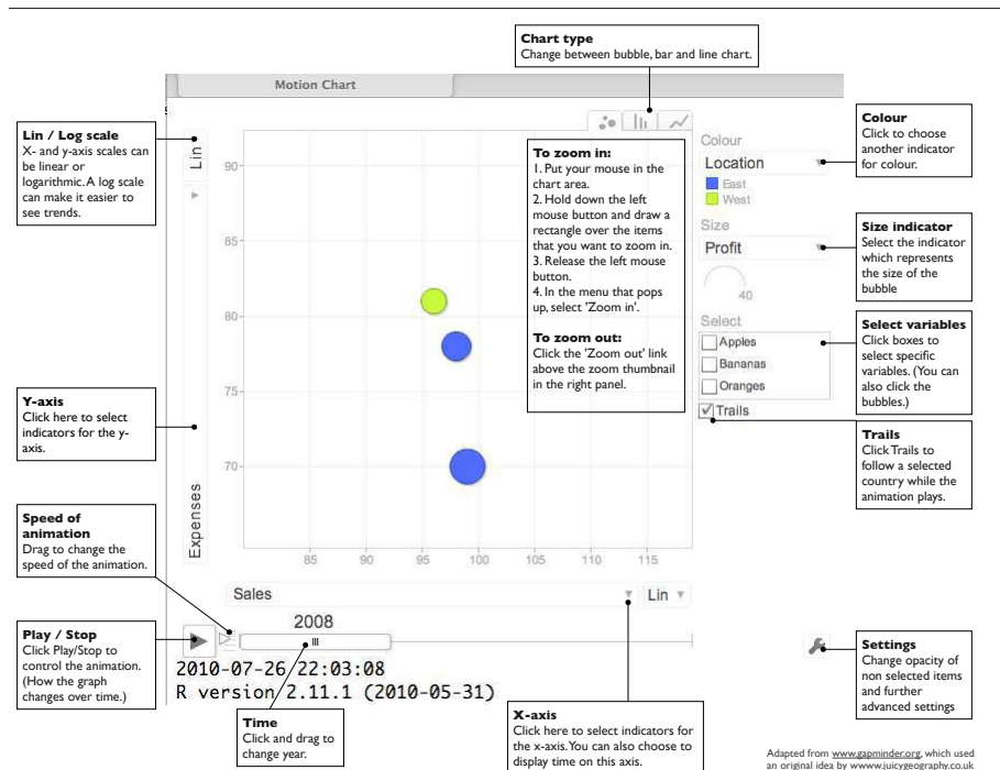
Figure 1: Overview of a Google Motion Chart. Screenshot of the output of plot(gvizMotionChart(Fruits, idvar='Fruit', timevar='Year'))
