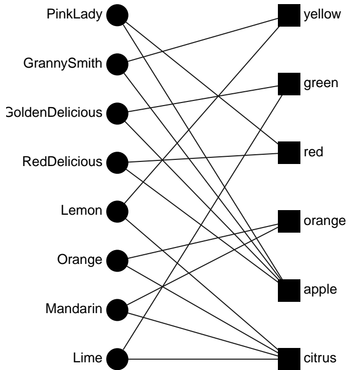
Figure 2: Bipartite graph
