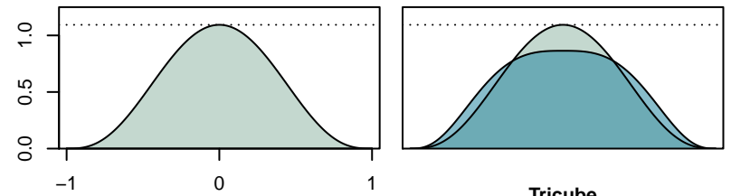
Tricube
