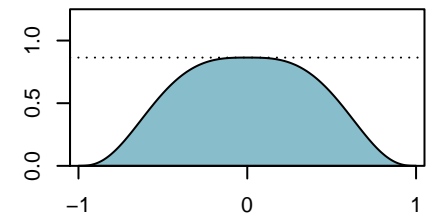
Tricube
