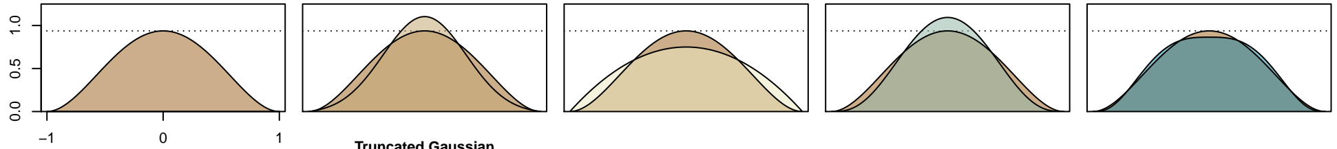
Truncated Gaussian
