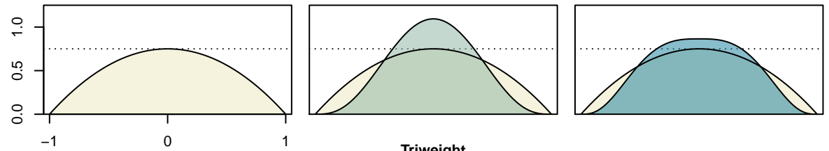
Triweight
