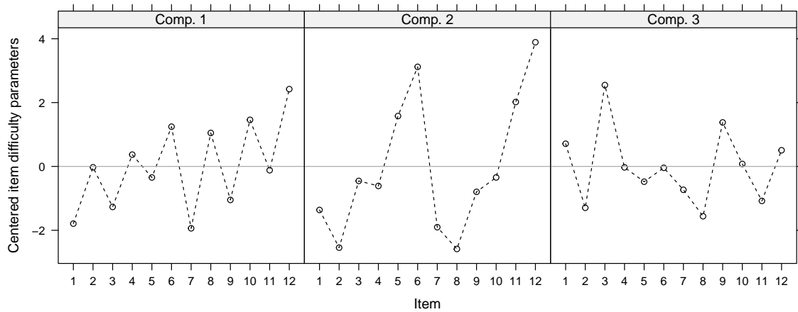
Figure 4: Item profiles for the 3-component Rasch mixture model on verbal aggression data. Items 1–6 pertain to situation S1 (bus), items 7–12 to situation S2 (train), each in the following order: want to curse, do curse, want to scold, do scold, want to shout, do shout.
