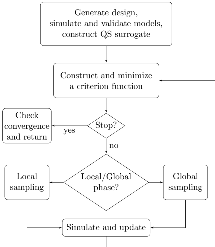
Figure 1: Algorithmic structure of function ql_e
