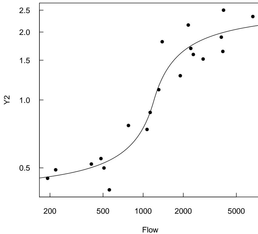
Figure 7. A flow-mixtura modeled using the sCurve function.
