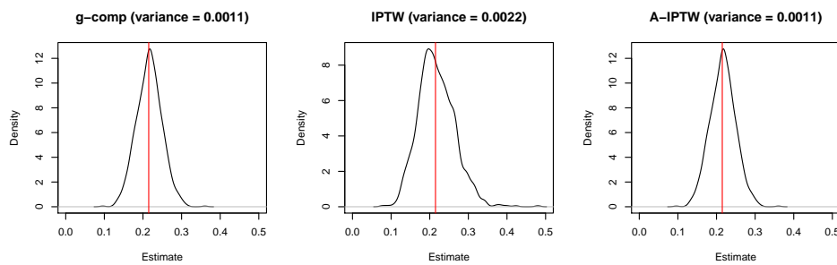
Figure 2: Density of various estimators considered.
