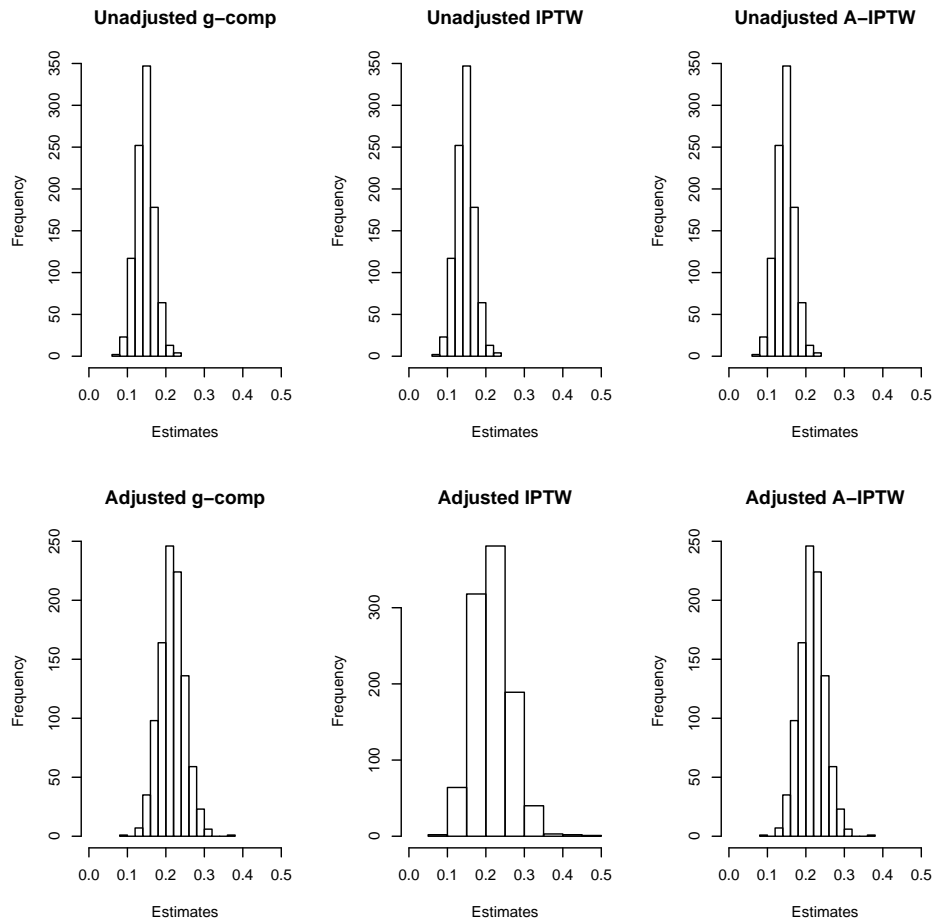
Figure 1: Histograms of various estimators considered.
