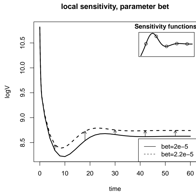
Figure 4: The sensitivity functions of \log V to parameter \text{bet} , as a function of time (upper right) are the (weighted) differences of the perturbed output (at \text{bet} = 2.2e-5 ) with the nominal output ( \text{bet} = 2e-5 ), main figure; the dots in the inset correspond to the arrows in the main figure.
