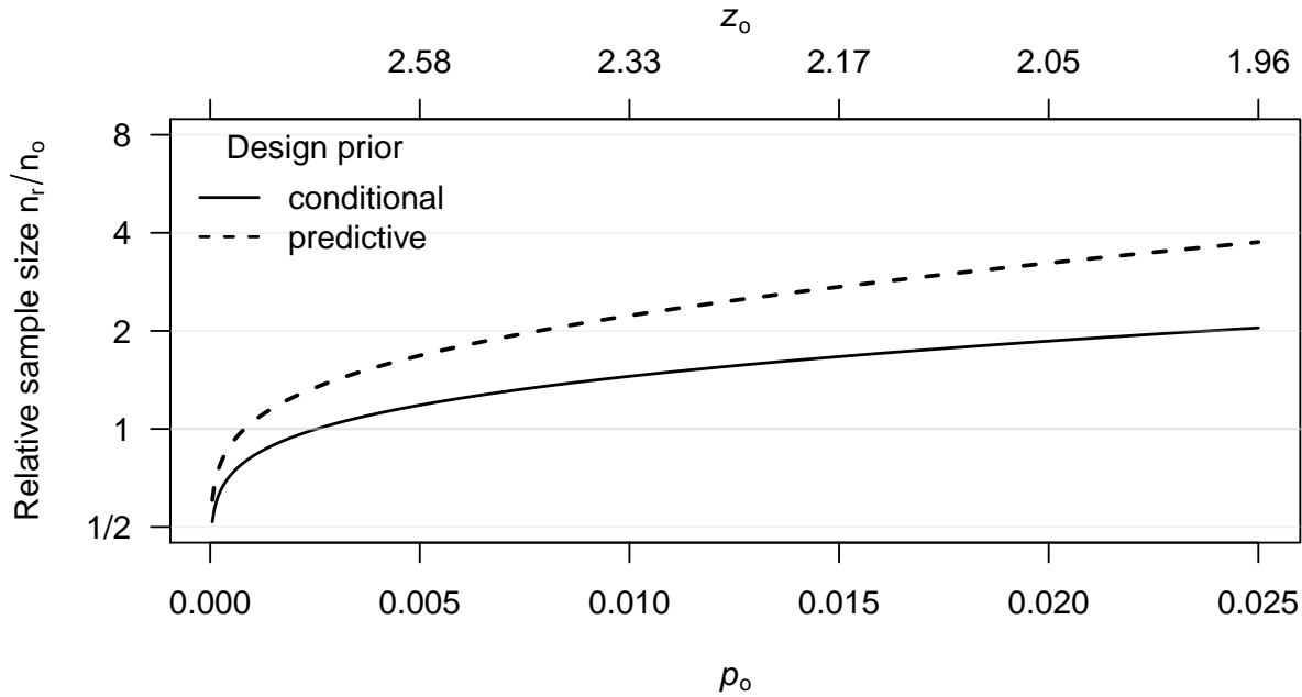
Figure 2: Relative sample size to achieve significance at the one-sided 2.5% level with 80% power as a function of (one-sided) p -value or z -value of original study.
