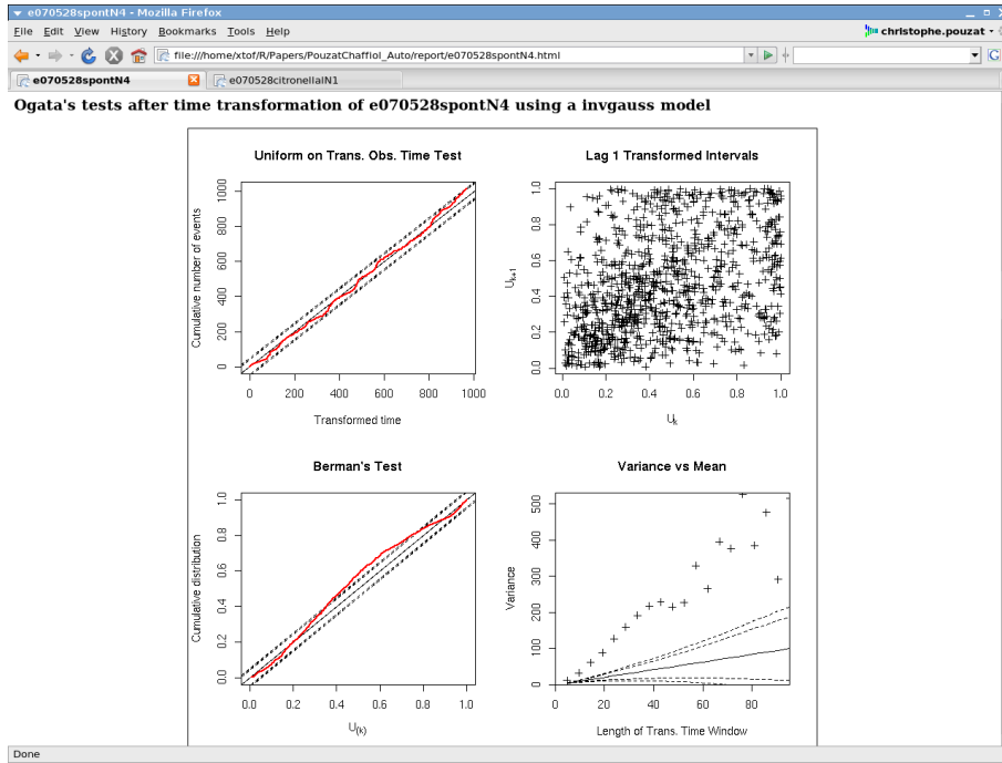
Figure 7: The equivalent of Fig. 5 this time with neuron 4 as it appears in the automatically generated HTML report.
