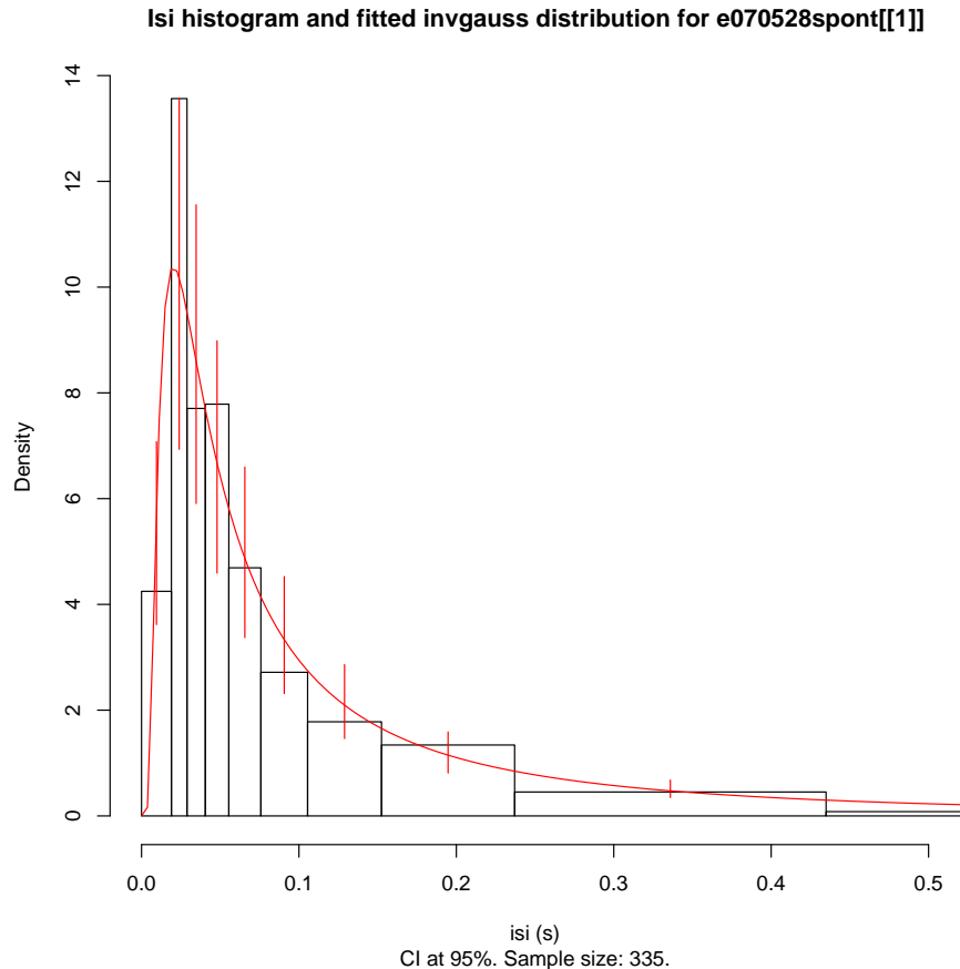
Figure 12: isi histogram (black rectangles) with superposed fitted inverse Gaussian density (red curve). The 10 histogram bins are set after the fit such that if the fit was good, 10% of the is would fall into each bin. Data of neuron 1, data set, e070528, spontaneous regime. For more details: ?isiHistFit .
