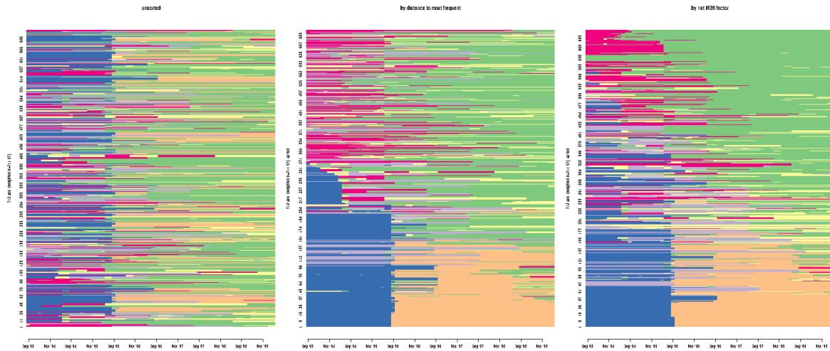
Figure 3: Unsorted and sorted full-sequence index plots.
