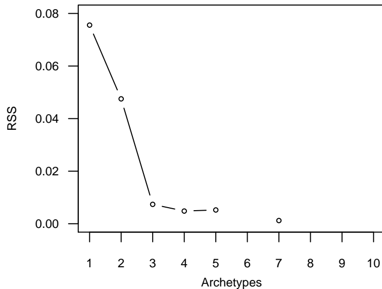
Figure 5: Screepplot of the residual sum of squares.
