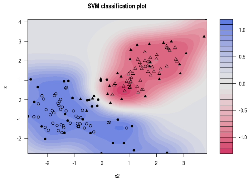
Figure 9: SVM classification plot.
