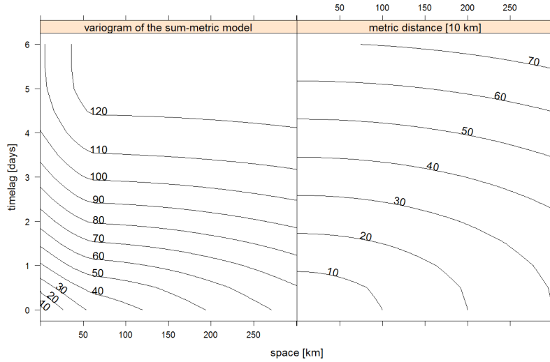
Figure 1: A contourplot showing how the spatio-temporal sum-metric variogram model (as estimated in the application below) and a metric distance relate to each other. Distances are rescaled by 1/5 for easy plotting.
