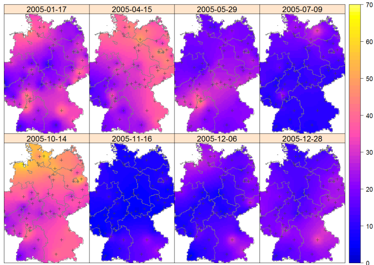
Figure 4: Spatio-temporal interpolation of daily mean PM_{10} concentrations using the sum-metric covariance model with the closest (approx. strongest correlated) 50 neighbouring spatio-temporal locations. The crosses indicate sampling locations. The cell size of the grid in UTM projection is 10 \text{ km} \times 10 \text{ km} .
