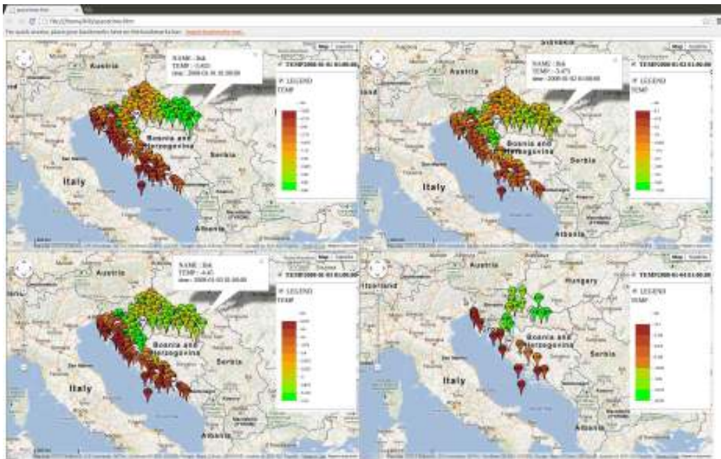
Figure 11: Plot STIDE.
