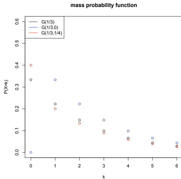
Figure 1.7: Mass probability function for zero-modified geometric distributions
