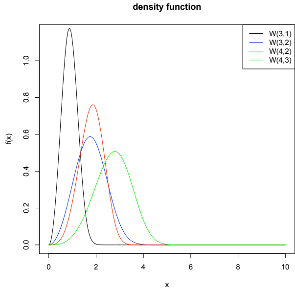
Figure 5.9: Density function for Weibull distributions
