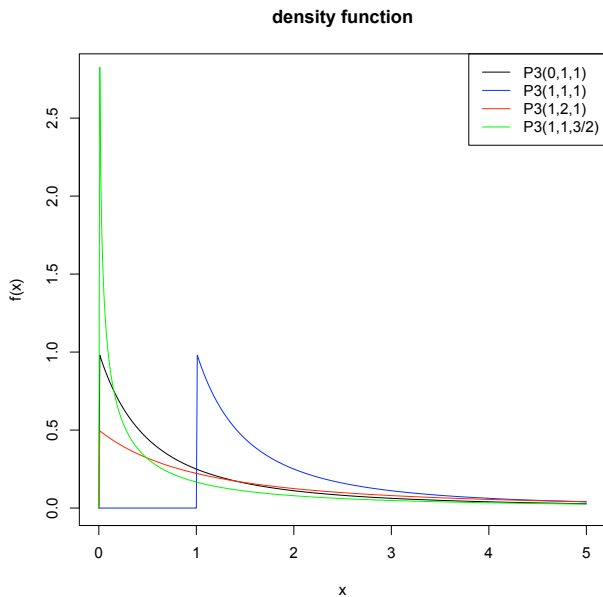
Figure 8.3: Density function for Pareto III distributions
