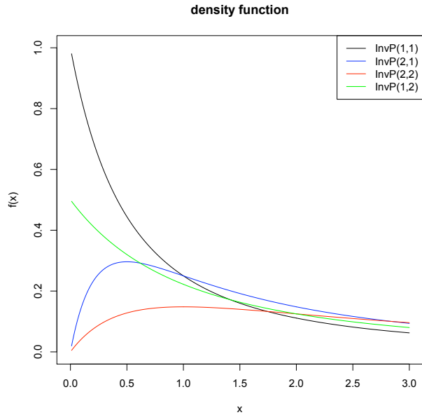
Figure 8.5: Density function for inverse Pareto distributions
