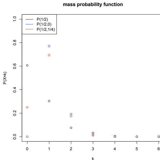
Figure 1.5: Mass probability function for zero-modified Poisson distributions
