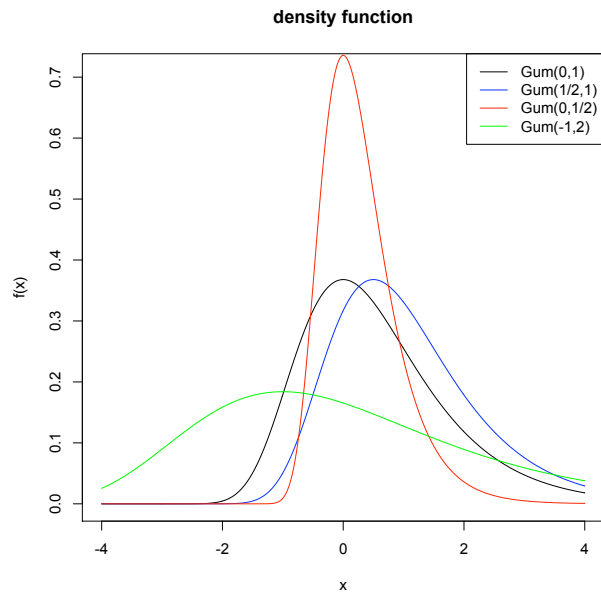
Figure 10.1: Density function for Gumbel distributions
