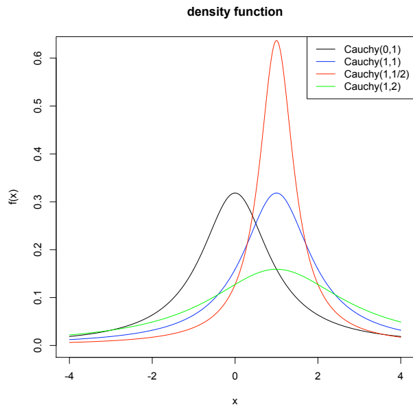
Figure 7.2: Density function for Cauchy distributions
