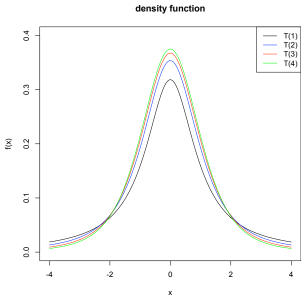
Figure 7.1: Density function for student distributions
