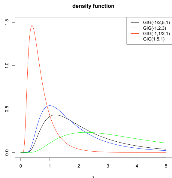
Figure 4.5: The density of generalized inverse Gaussian distributions
