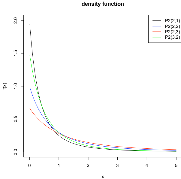
Figure 8.2: Density function for Pareto II distributions
