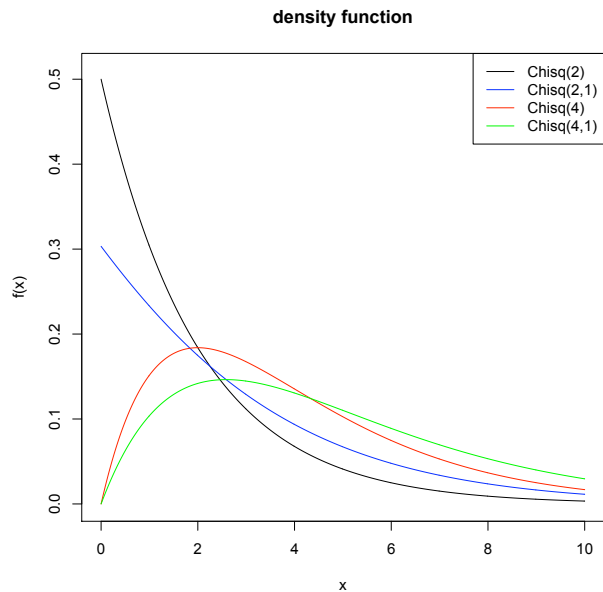
Figure 6.3: Density function for non central chi-squared distributions
