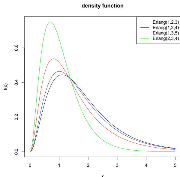
Figure 5.5: Density function for generalized Erlang distributions
