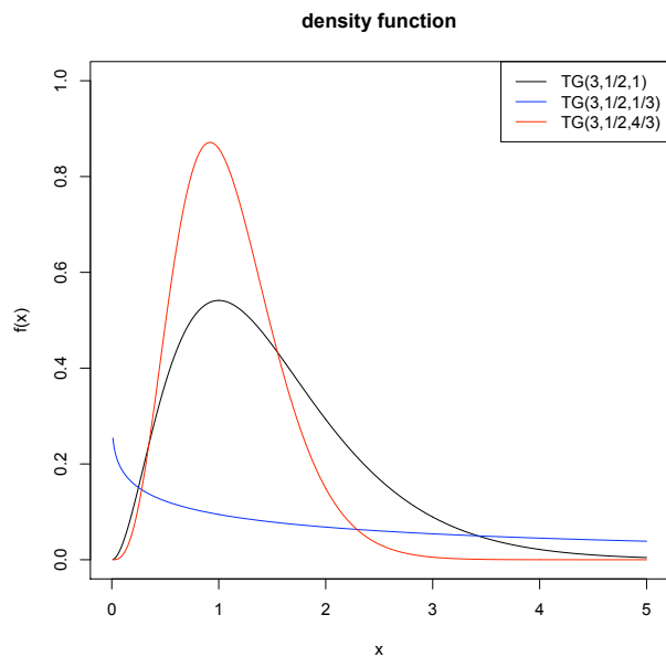
Figure 5.7: Density function for transformed gamma distributions
