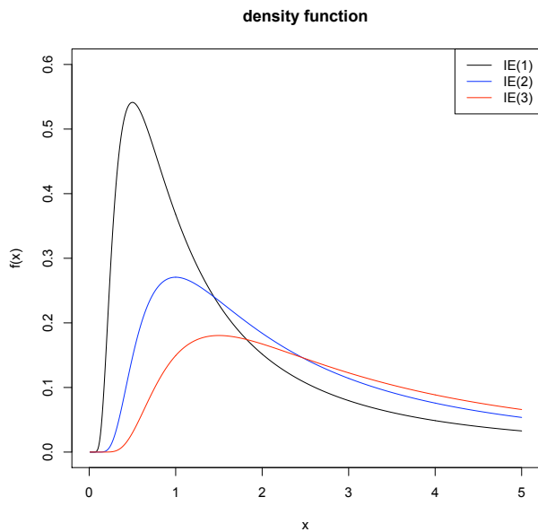
Figure 5.3: Density function for inverse exponential distributions
