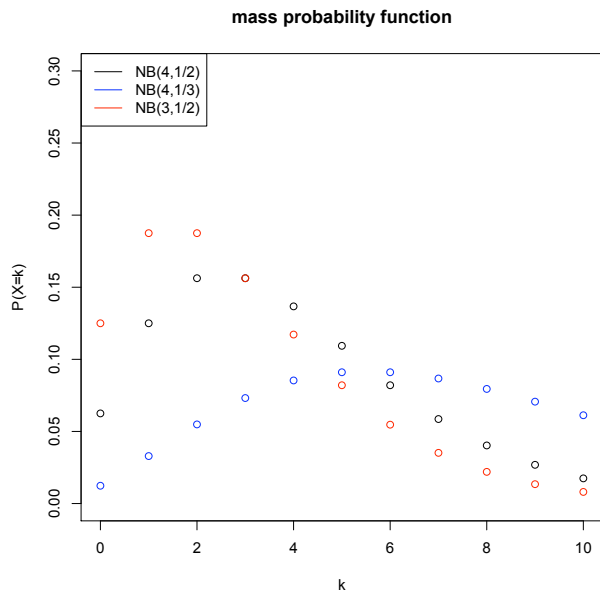
Figure 1.8: Mass probability function for negative binomial distributions
