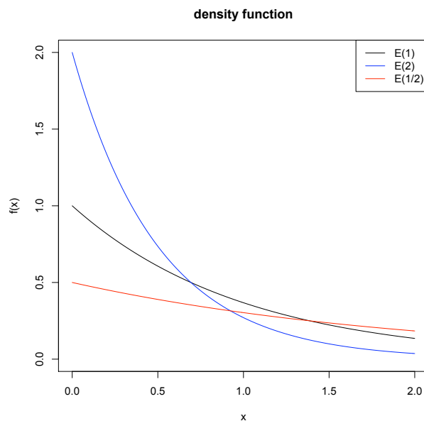
Figure 5.1: Density function for exponential distributions
