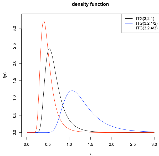
Figure 5.8: Density function for inverse transformed gamma distributions
