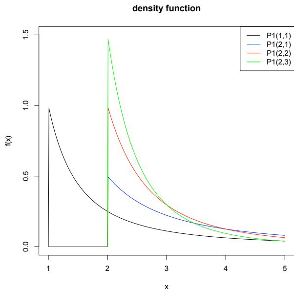
Figure 8.1: Density function for Pareto I distributions
