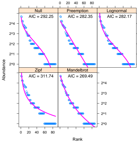
Figure 4: Ranked abundance distribution models for a random plot (no. 42). The best model has the lowest AIC.
