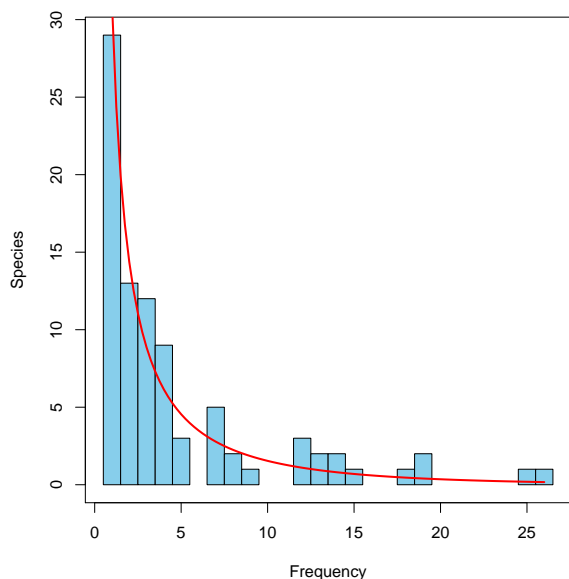
Figure 3: Fisher’s log-series fitted to one randomly selected site (42).
